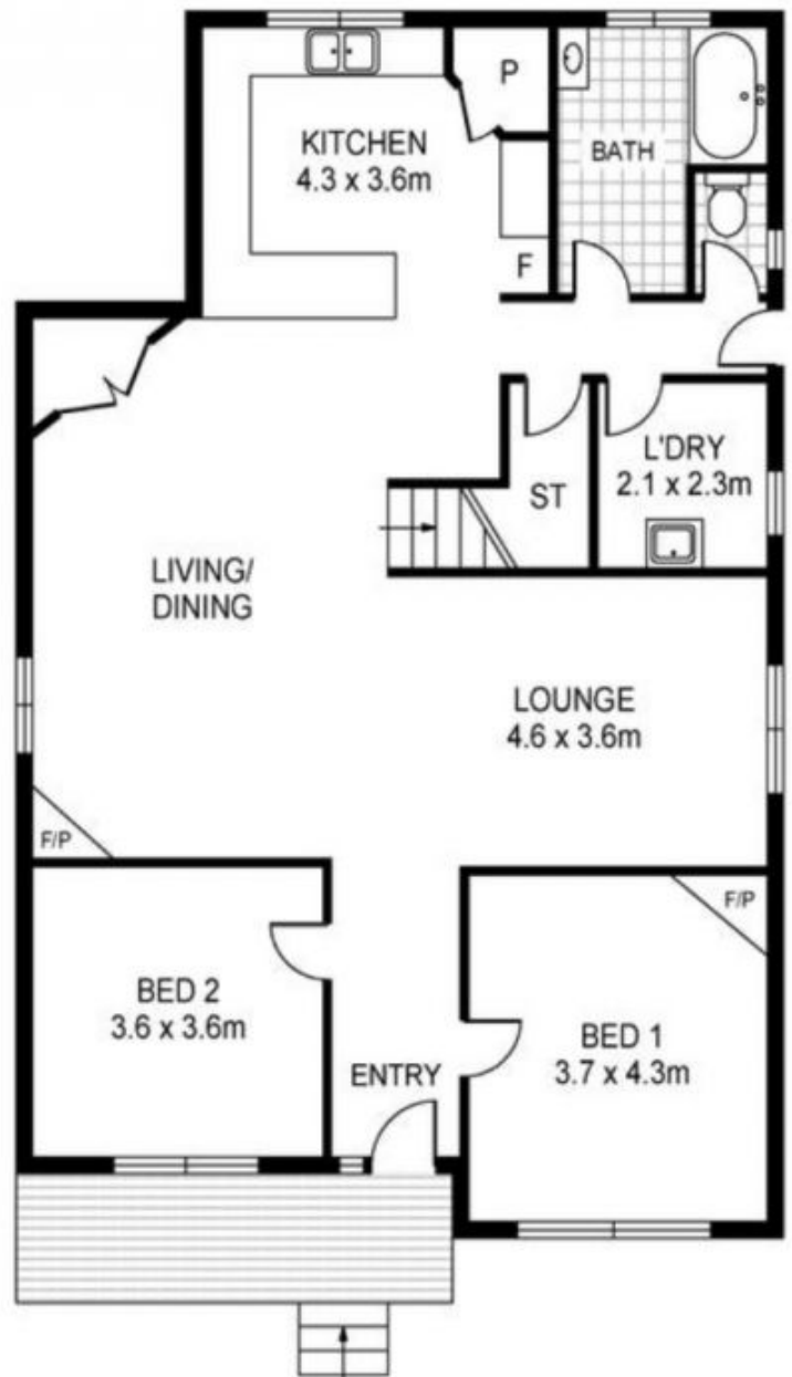
GROUND FLOOR
